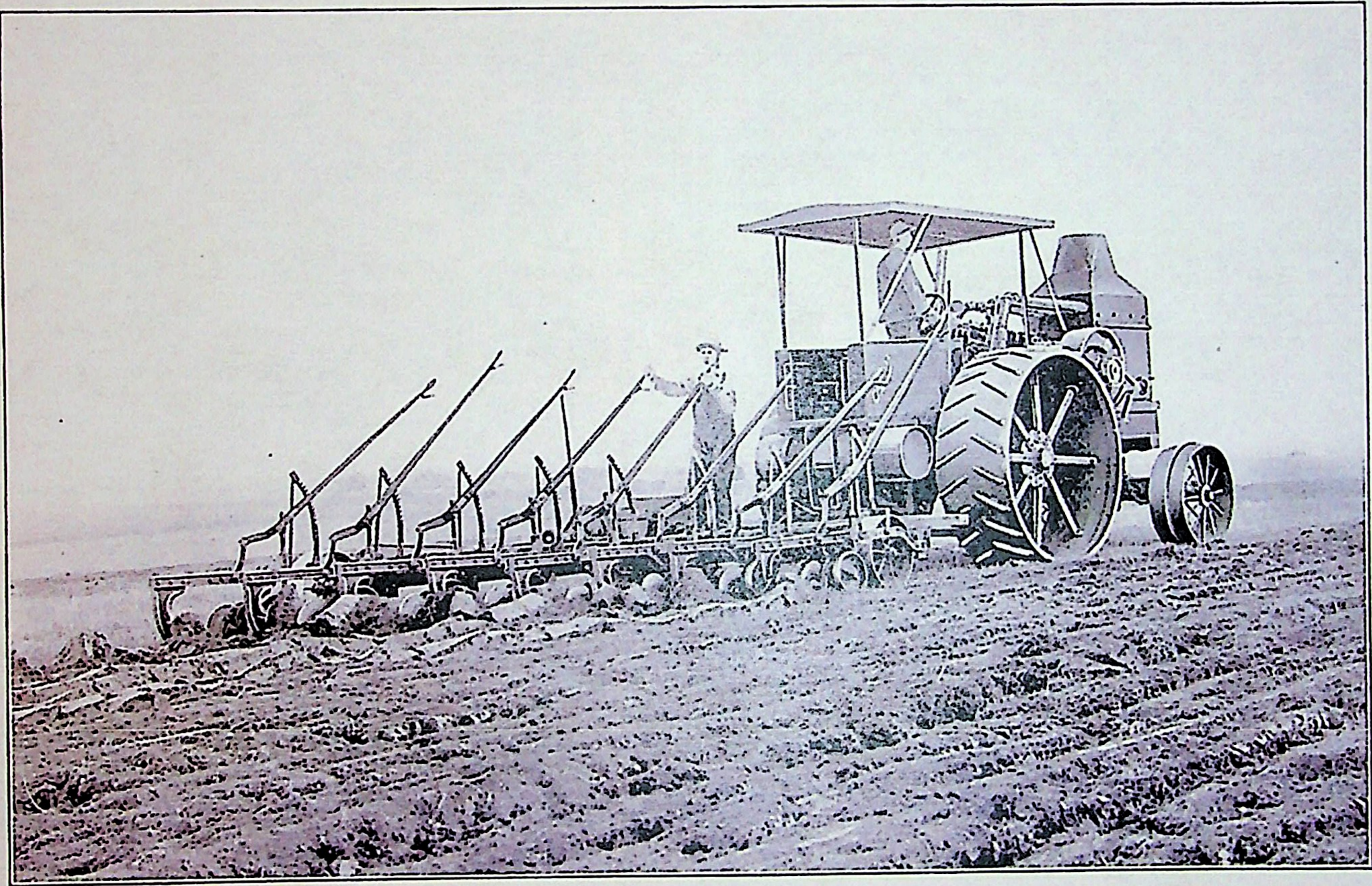
30-60 h. p. Rumely Tractor Plowing with Eight-Bottom Rumely Engine Gang Plow
